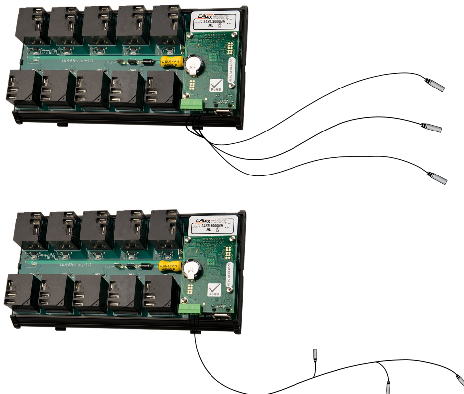
Figure 2.2g - Direct Connection (Star) and Daisy Chain Connection(Linear)
