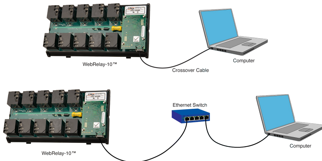
Figure 2.2a - Network Connection
