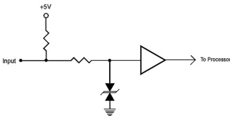
Figure 2.2d - Input Schematic
