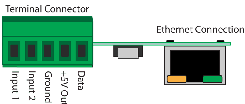
Figure 2.2c - Connector Pinout
